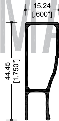
9756 MARCO 1 3/4"
