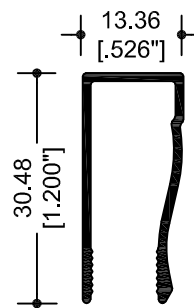
13563 MARCO 1 1/4"
