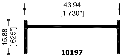
10197 JAMBA LATERAL
