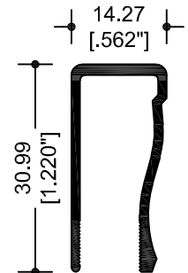
9525 MARCO 1 1/4"
