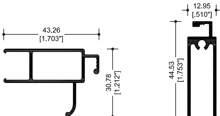
7112 VERTICAL MOSQUITERO
