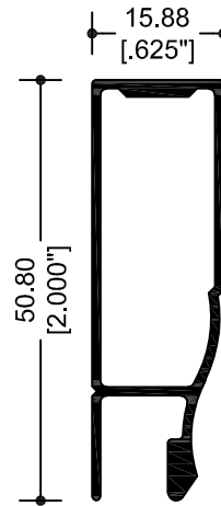
10103 MARCO 2"
